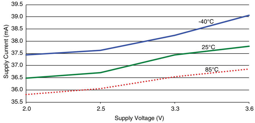
Figure 15: HumRC™ Series Transceiver TX Current vs. Supply Voltage at Max Power - HUM-900-RC
