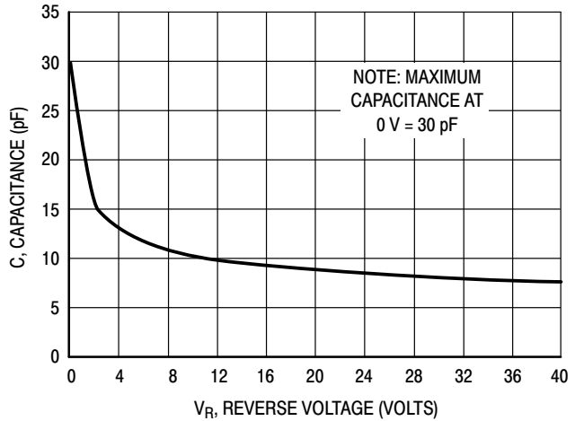
Figure 7. Maximum Capacitance
