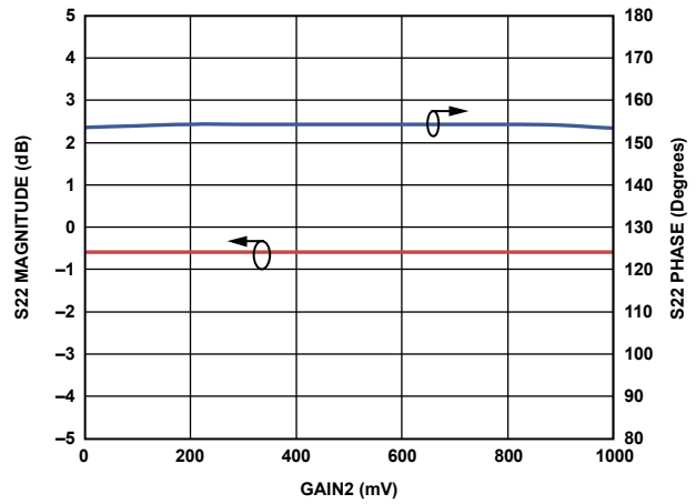
Figure 45. S_{22} (re: 100\ \Omega ) Magnitude and Phase vs. V_{GAIN} for VGA2
