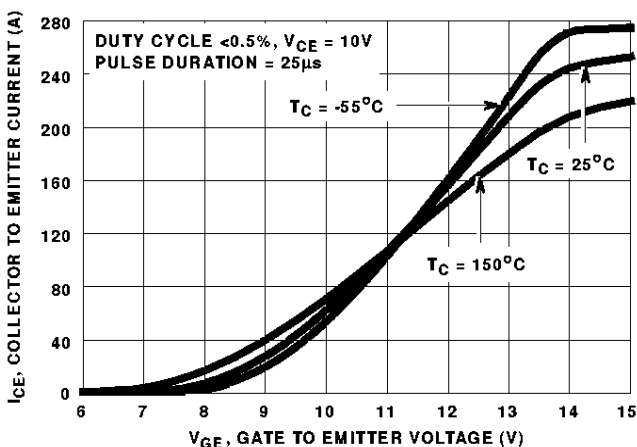
FIGURE 11. TRANSFER CHARACTERISTICS
