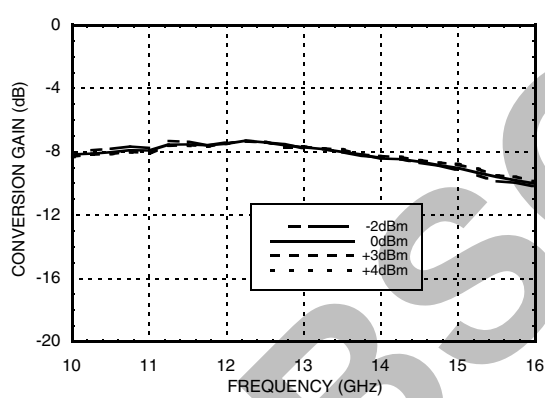
Upconverter LSB, IF = 3 GHz Conversion Gain vs. LO Drive
