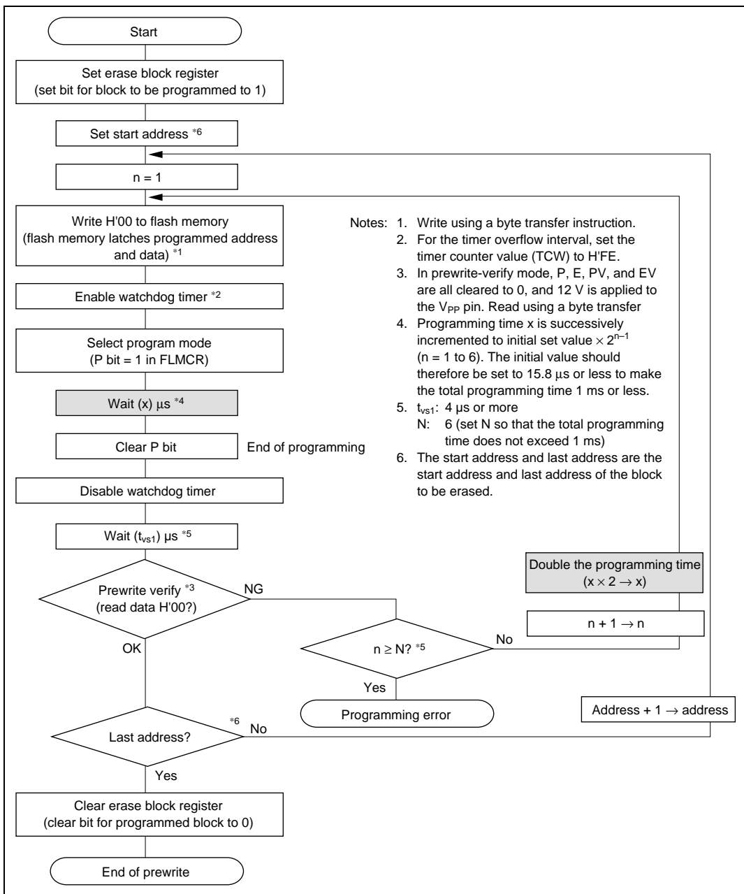
Figure 6.15 Prewrite Flowchart
