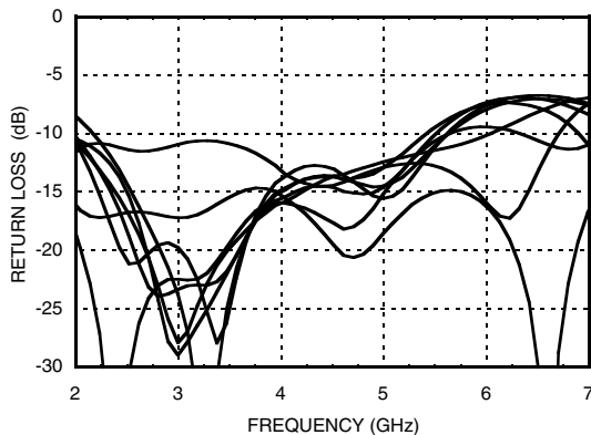
Output Return Loss, Major States Only
