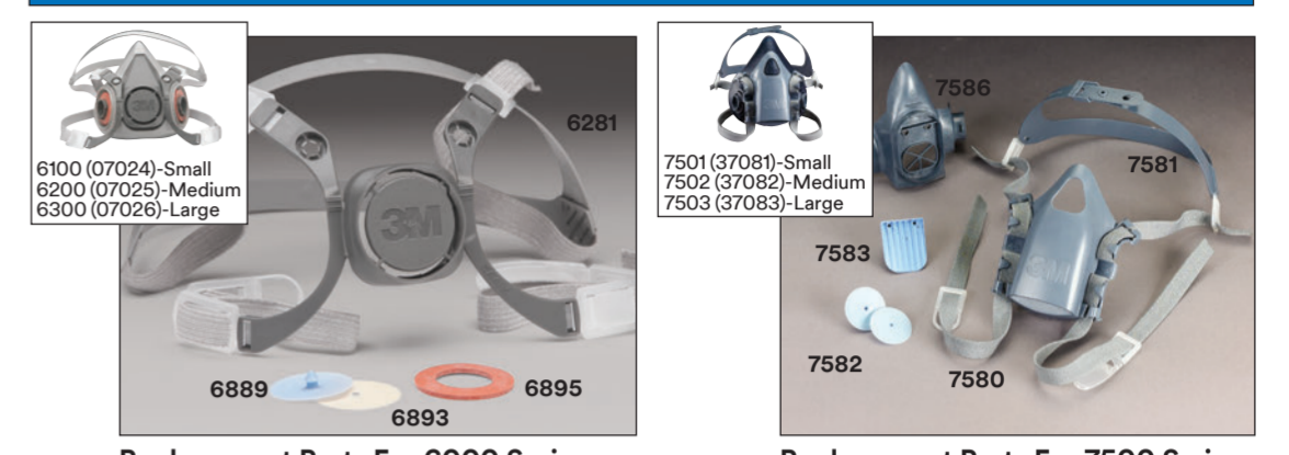
Replacement Parts For 6000 Series Half Facepiece Respirators 6281 Head Harness Assembly 6859 Exhalation Valve 6893 Inhalation Valve 6895 Inhalation Gasket
