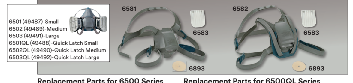
Replacement Parts for 6500 Series Half Facepiece Respirators 6581 Standard Head Harness 6583 Exhalation Valve 6893 Inhalation Valve
