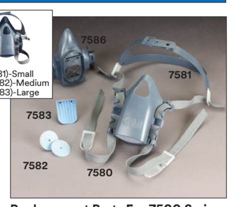
Replacement Parts For 7500 Series Half Facepiece Respirators 7580 Replacement Strap 7581 Head Harness Assembly 7582 Inhalation Valve 7583 Exhalation Valve 7586 Cartridge/Filter Holder (includes valves, not shown)
