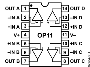
Figure 1. 14-Lead PDIP (N-14) (P Suffix)
