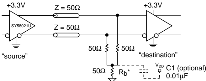
Figure 14. Three-Resistor "Y-Termination"
