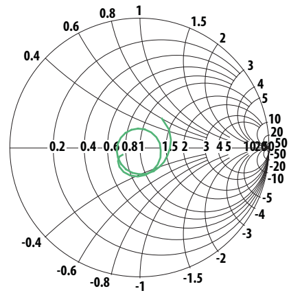
Figure 21. Ant Port Impedance in Rx Band
