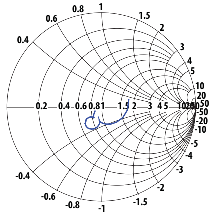
Figure 19. Rx Port Impedance in Rx Band
