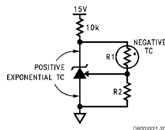
FIGURE 7. Output Voltage has Positive Temperature Coefficient (TC) if R1 has Negative TC
