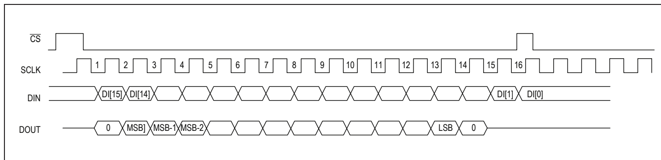
Figure 2c. External Clock Mode Timing Diagram with CHAN_ID=0
