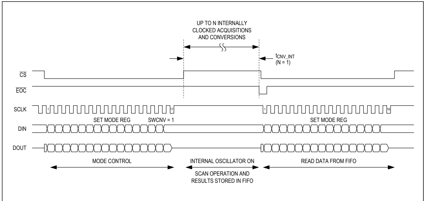
Figure 7. Internal Conversions with SWCNV
