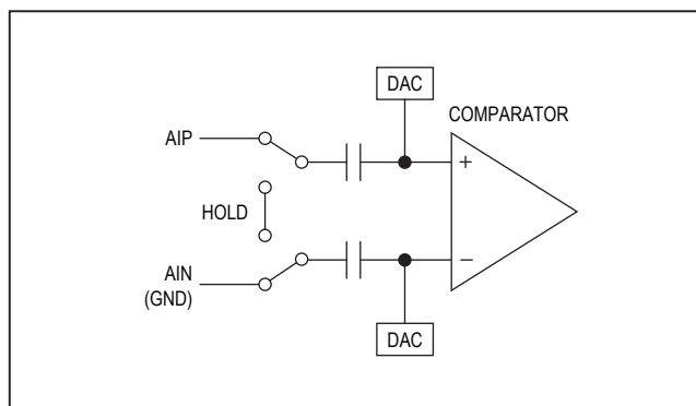
Figure 3. Equivalent Input Circuit
