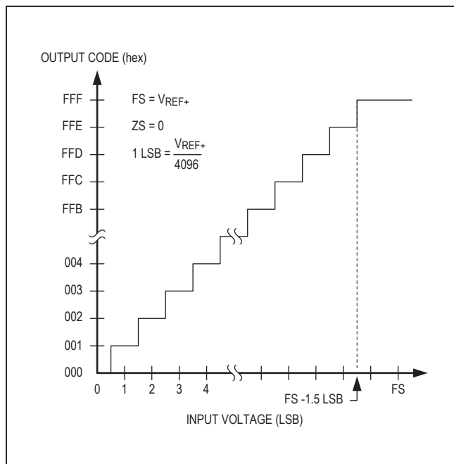
Figure 4. Unipolar Transfer Function for 12-Bit Resolution
