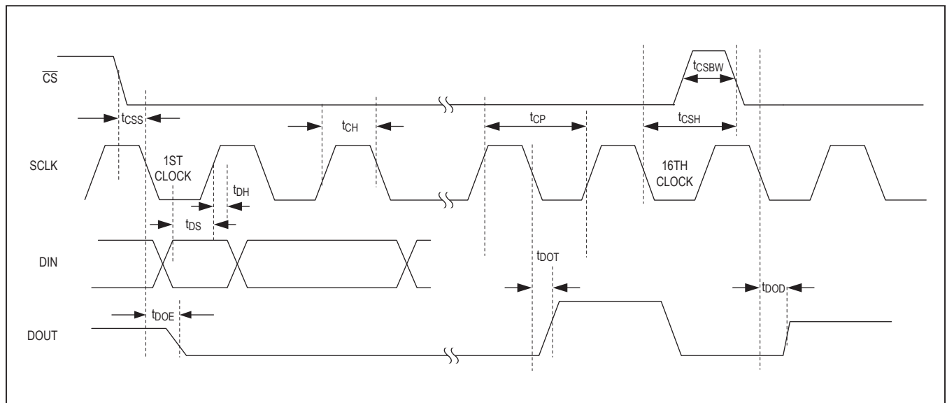
Figure 1. Detailed Serial-Interface Timing Diagram
