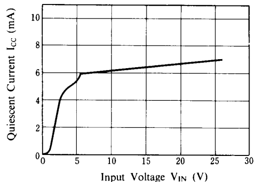
NJM2930F05/L05 I_{cc}-V_{IN}
