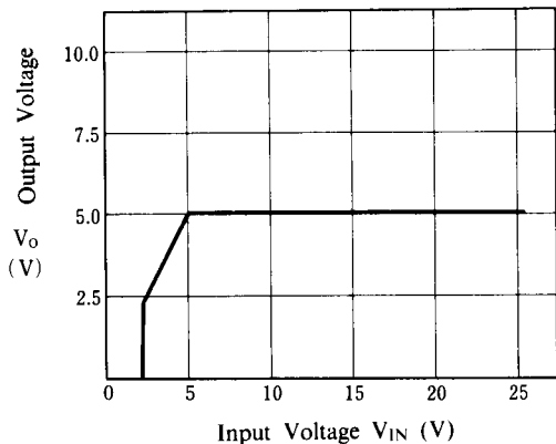
NJM2930F05/L05 Output Voltage
