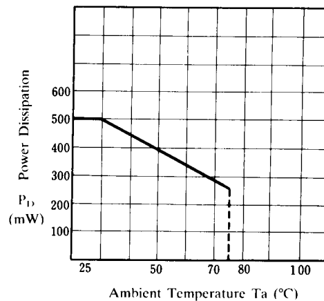
NJM2930L (TO-92)
