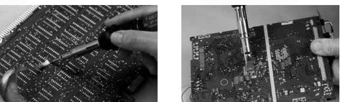
Solder Desolder
