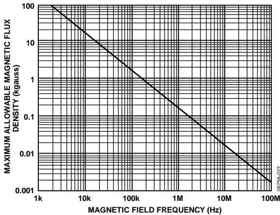
Figure 25. Maximum Allowable External Magnetic Flux Density
