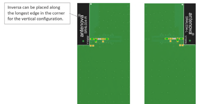
Vertical placement
