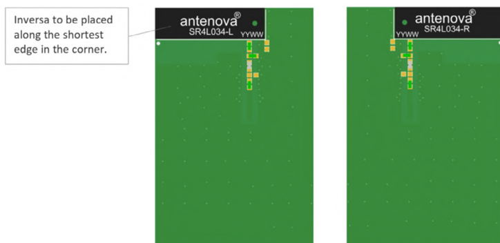
Horizontal placement
