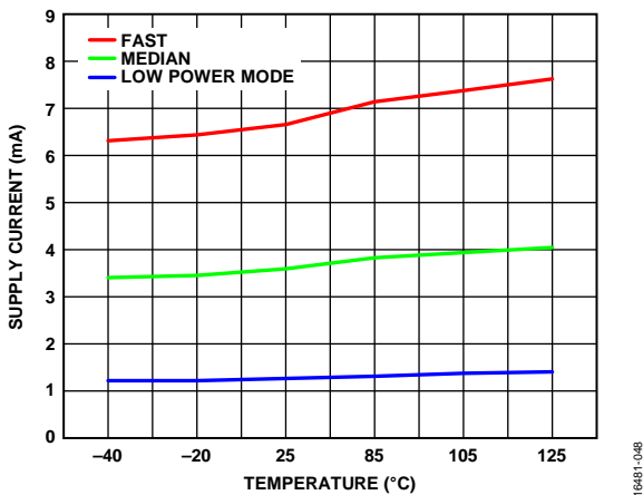
Figure 48. Supply Current vs. Temperature, AVDD1
