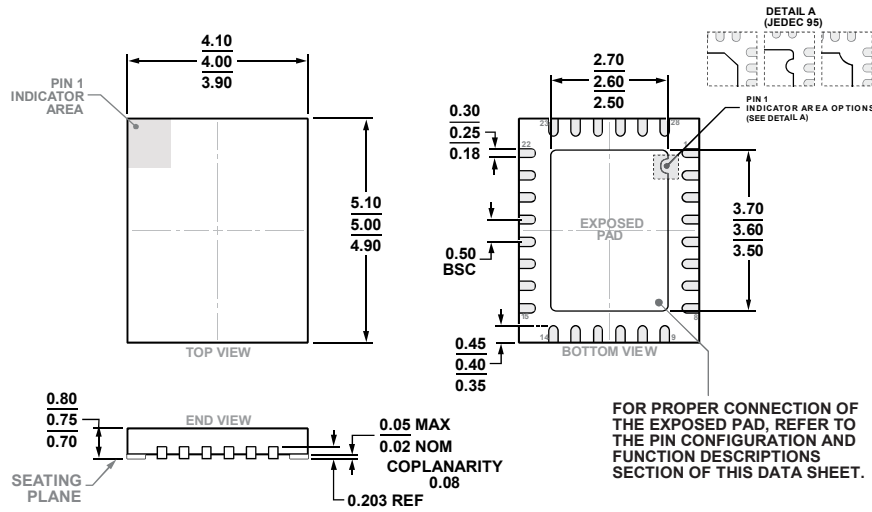
COMPLIANT TO JEDEC STANDARDS MO-220-WGHD-3 Figure 101. 28-Lead Lead Frame Chip-Scale Package [LFCSP] 4 mm x 5 mm Body and 0.75 mm Package Height (CP-28-12) Dimensions shown in millimeters
