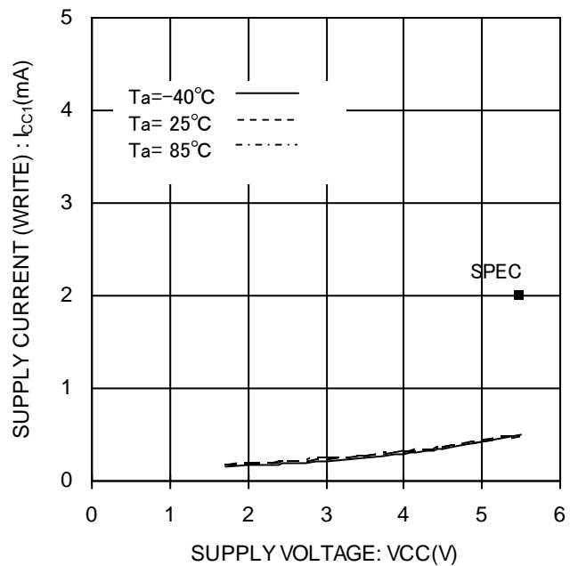
Figure 15. Supply current (WRITE) I_{CC1}(\text{WRITE}, f_{SK}=3\text{MHz})
