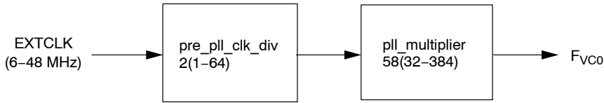
Figure 20. PLL Dividers Affecting VCO Frequency
