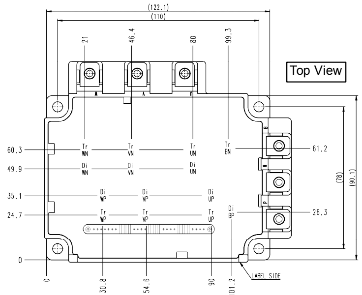
PM100RL1A120 350G
