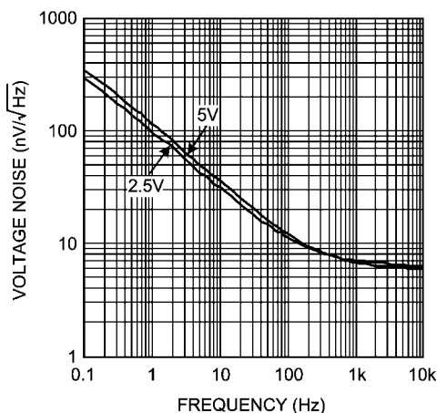
30010839 Input Referred Voltage Noise vs. Frequency
