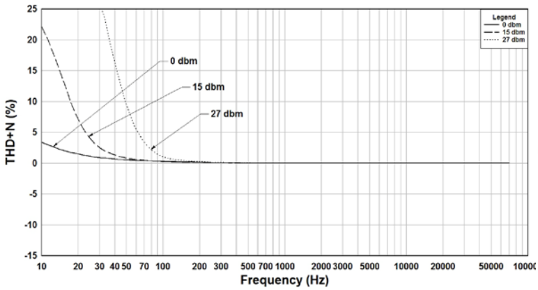
108K Rs=1500, RI=600 THD+N
