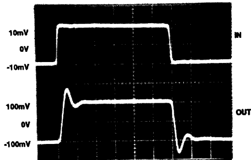
SMALL SIGNAL RESPONSE Input: 10mV/Div. Output: 100mV/Div.
