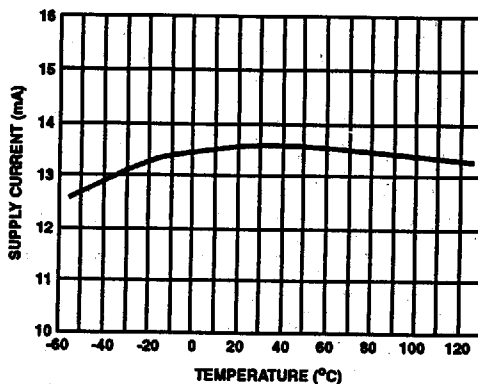
FIGURE 19. SUPPLY CURRENT vs TEMPERATURE
