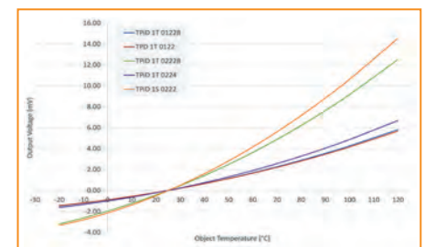
Fig 9: Sensitivity curves
