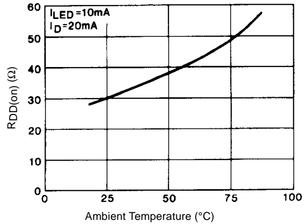
Figure 4. Typical On-Resistance
