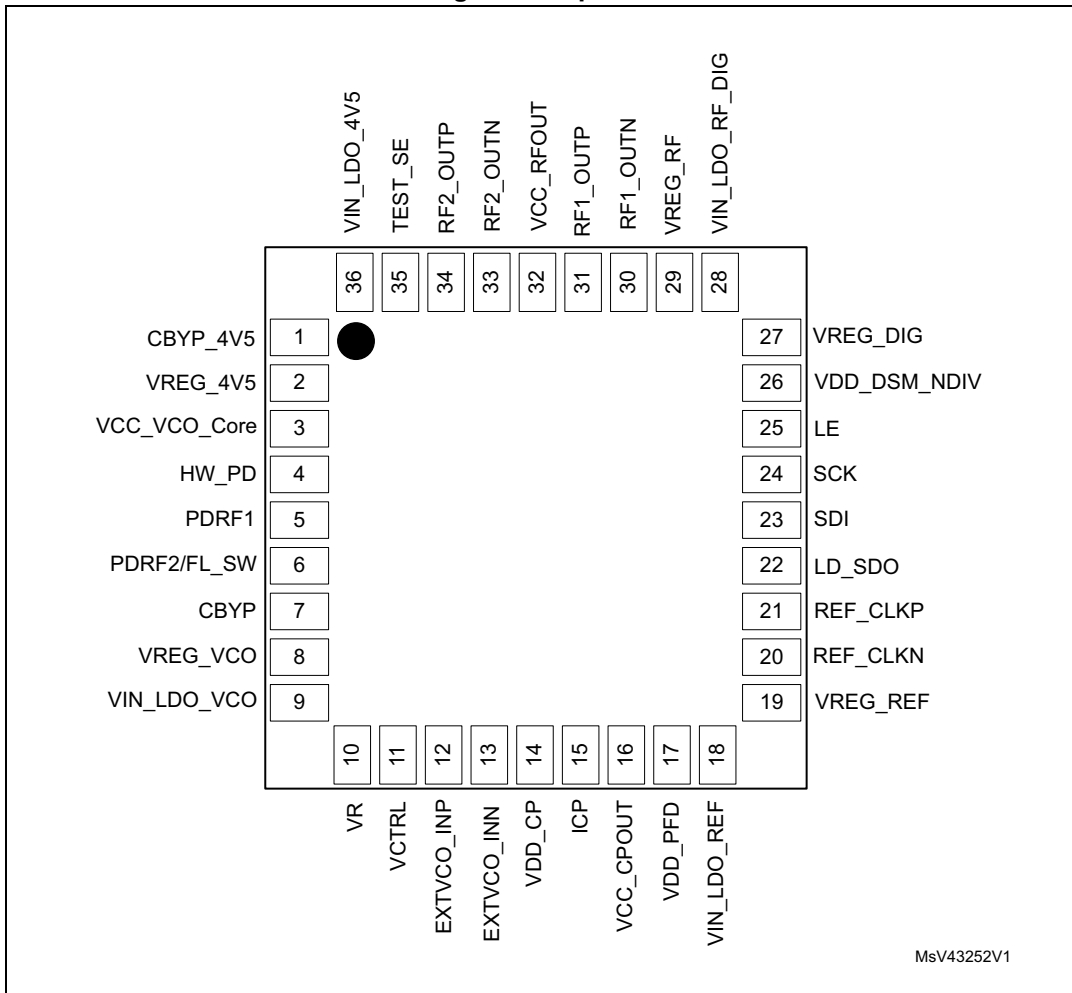
Figure 2. Top view
