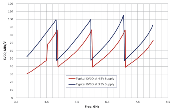
Figure 8. Average K_{\text{VCO}} over VCO frequency and supply
