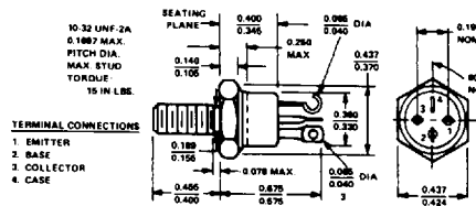
TO-111 (ISOLATED)
