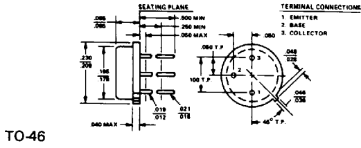
TO-46
