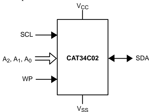
Figure 1. Functional Symbol
