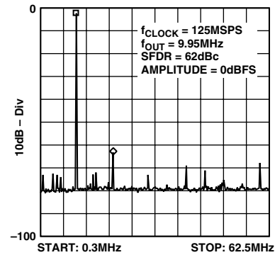
Figure 36. Single-Tone SFDR
