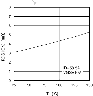
RDS(ON)-Tc characteristics (typical) ID=58.5A, VGS=10V
