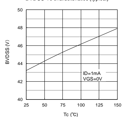
BVDSS-Tc characteristics (typical) ID=1mA, VGS=0V
