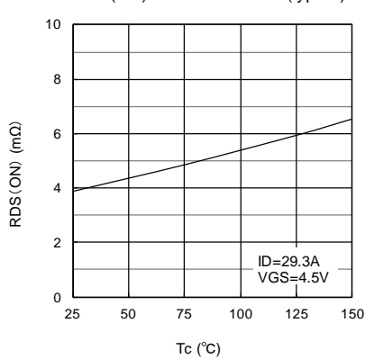
RDS(ON)-Tc characteristics (typical) ID=29.3A, VGS=4.5V
