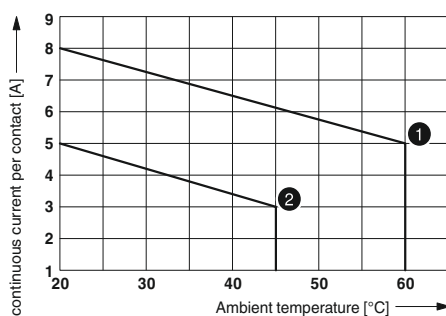
Contact derating
