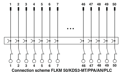
Connection scheme FLKM 50/KDS3-MT/PPA/AN/PLC
