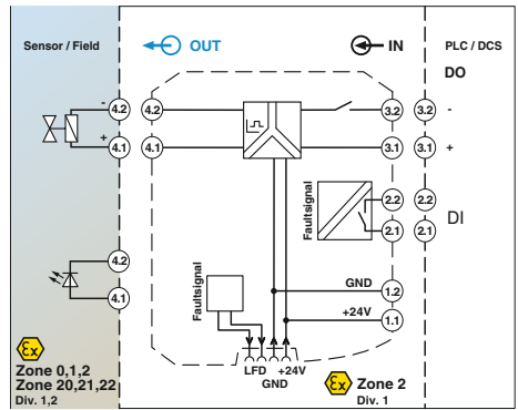
Solenoid driver, 25.1 mA current limitation with line fault detection
