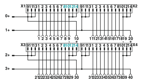
Connection scheme FLKM 50/ 4-FLK14/PA-MODI-TSX/Q
