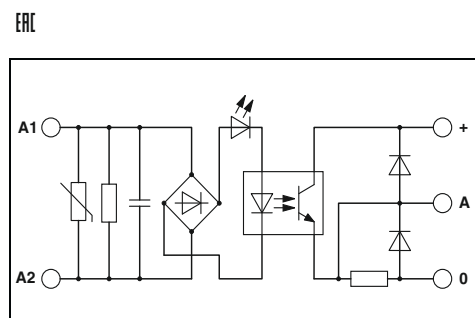
Solid-state input relay max. 100 mA
