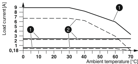
Derating curve for ELR H3...24DC...
