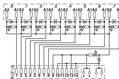
Connection scheme for RIF-1-V8/PT/FLK14/OUT
