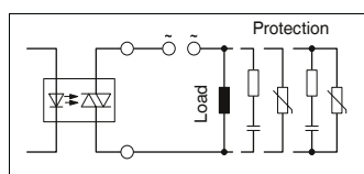
Figure 7: Protective circuit with AC voltage output
