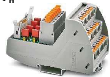
Fuse module for DeltaV for 8 channels With Push-in connection
