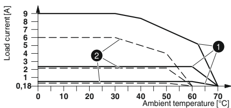
Derating curve for ELR H3...230AC...
