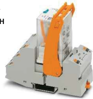
2-changeover-contact octal relay module with Push-in connection and manual operation
