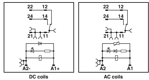
1-changeover-contact relay module with Push-in connection and manual operation
