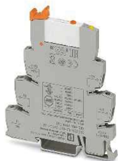
1-N/O-contact relay module with manual operation and additional floating terminal point
