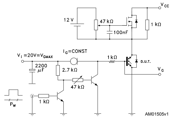
Figure 25. Gate charge test circuit
