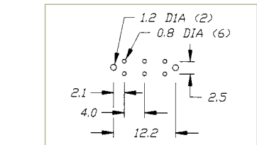
P.C. MOUNTING
