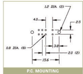
P.C. MOUNTING
