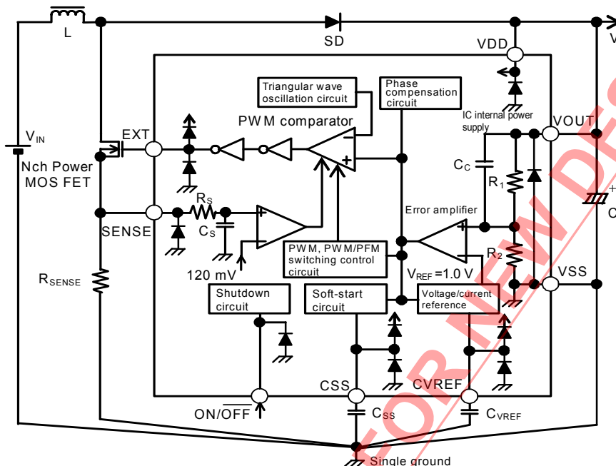
Figure 14 Output Voltage Fixed Output Type
