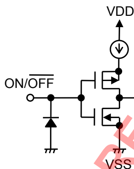
Figure 11 ON/OFF Pin Structure
