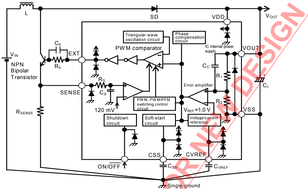
Figure 16 Output Voltage Fixed Output Type
