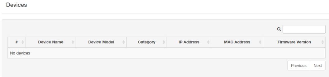
Figure 117: Tools > IXM
