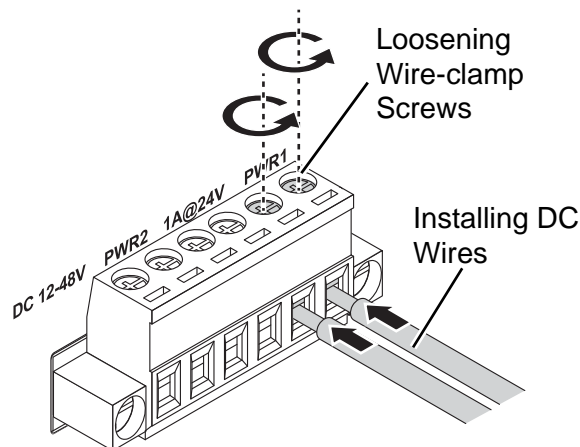
Figure 28: Installing DC Wires in a Terminal Block
