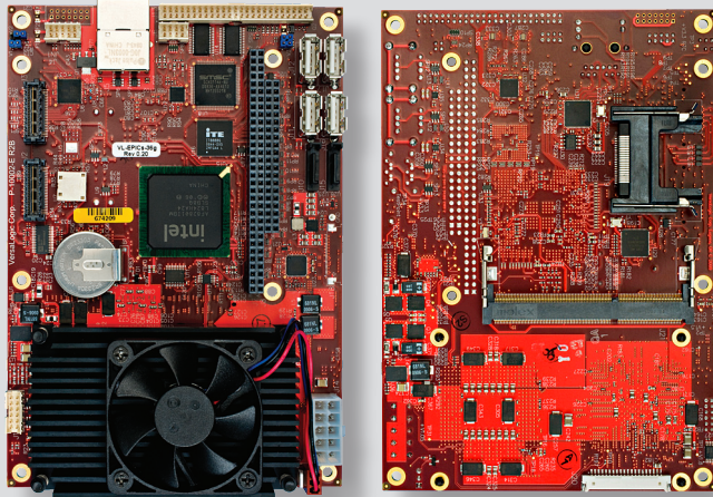
VL-EPICs-36S (Top)
