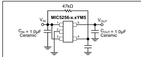
FIGURE 4-1: Low-Noise Fixed Voltage Application.
