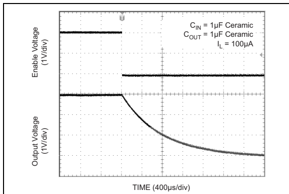
FIGURE 2-21: Shutdown Delay.
