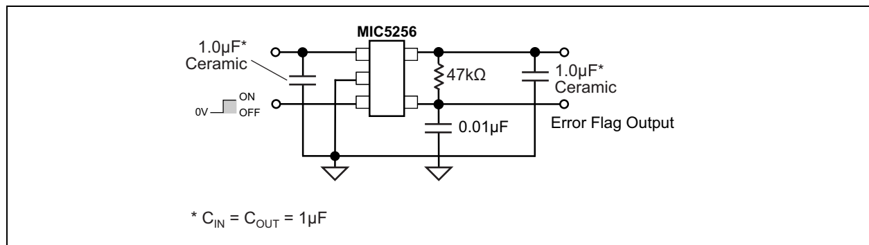
FIGURE 1-1: Test Circuit.
