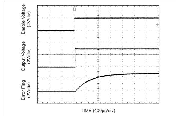
FIGURE 2-22: Error Flag Start-Up (see Figure 1-1 ).
