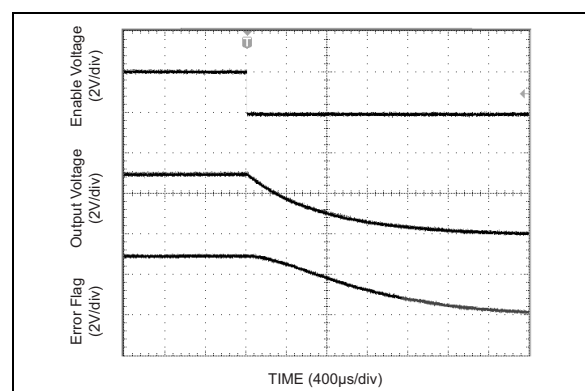
FIGURE 2-23: Error Flag Shutdown (see Figure 1-1 ).
