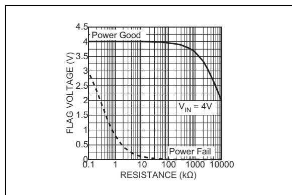
FIGURE 2-17: Error Flag Pull-Up Resistor.
