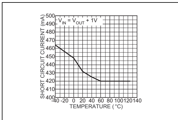
FIGURE 2-14: Short-Circuit Current.
