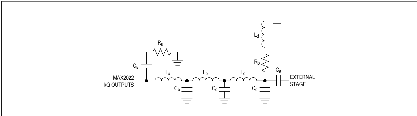
Figure 6. Baseband Port Typical Filtering and DC Return Network
