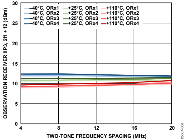
Figure 70. Observation Receiver IP3, 2f_1 + f_2 vs. Two-Tone Frequency Spacing, Both Tones at -13 dBFS, f_2 = 2 MHz
