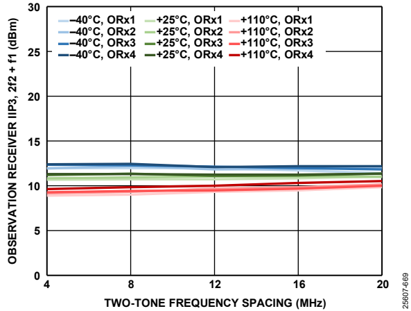
Figure 71. Observation Receiver IP3, 2f_2 + f_1 vs. Two-Tone Frequency Spacing, Both Tones at -13 dBFS, f_2 = 2 MHz
