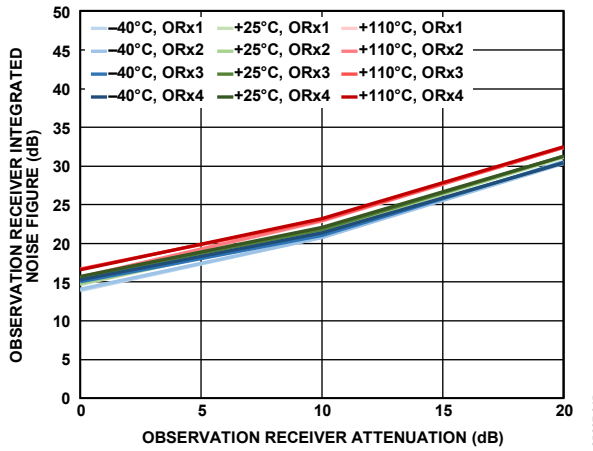
Figure 47. Observation Receiver (ORx) Integrated Noise Figure vs. Observation Receiver Attenuation, 141 MHz Bandwidth, Sample Rate = 153.6 MSPS, Integration Bandwidth = 500 kHz to 70.5 MHz
