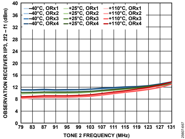
Figure 69. Observation Receiver IP3, 2f_2 - f_1 vs. Tone 2 Frequency, Both Tones at -13 dBFS, f_1 = f_2 + 2 MHz
