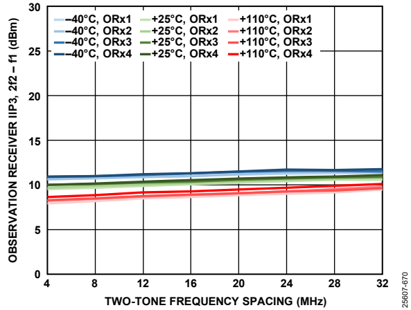
Figure 72. Observation Receiver IP3, 2f_1 - f_2 vs. Two-Tone Frequency Spacing, Both Tones at -13 dBFS, f_2 = 2 MHz
