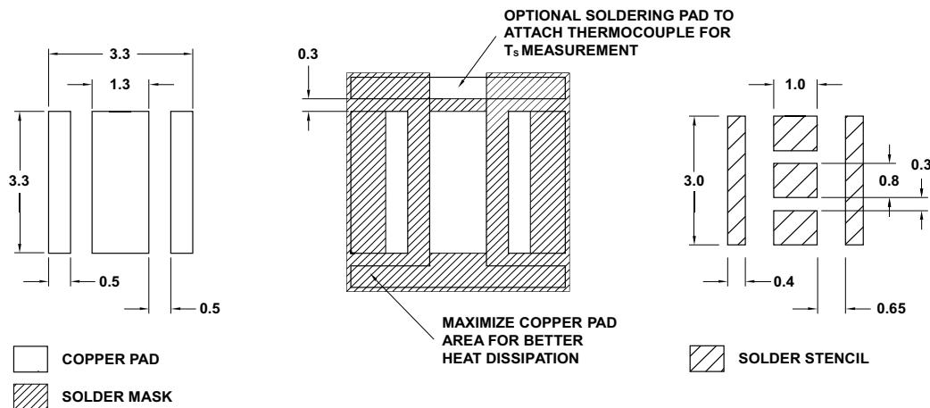
Figure 18: Recommended Soldering Land Pattern
