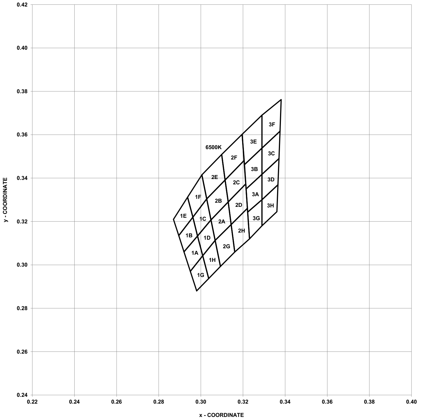
Figure 2: Chromaticity Diagram
