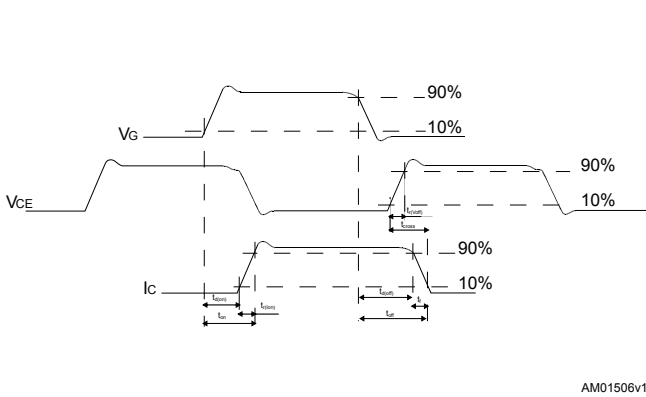
Figure 29. Switching waveform
