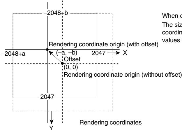
Figure 3.16 Rendering Coordinates
