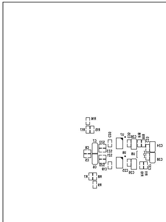
Figure 6. Silkscreen Bottom
