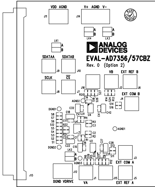
Figure 5. Silkscreen Top
