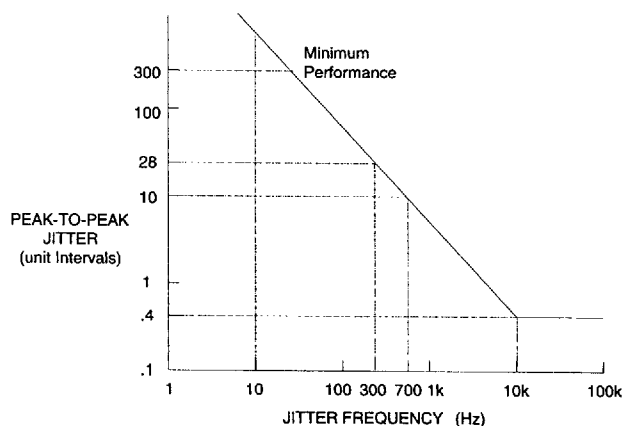
Figure 7. - Input Jitter Tolerance of Receiver
