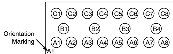
CM1426-08CP 20 Bump CSP Package
