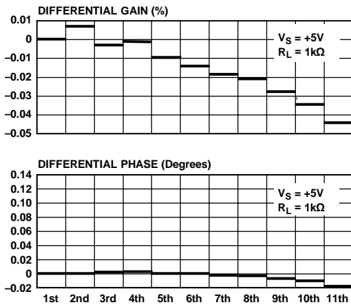
Figure 37. Differential Gain and Differential Phase, R_L = 1k\Omega
