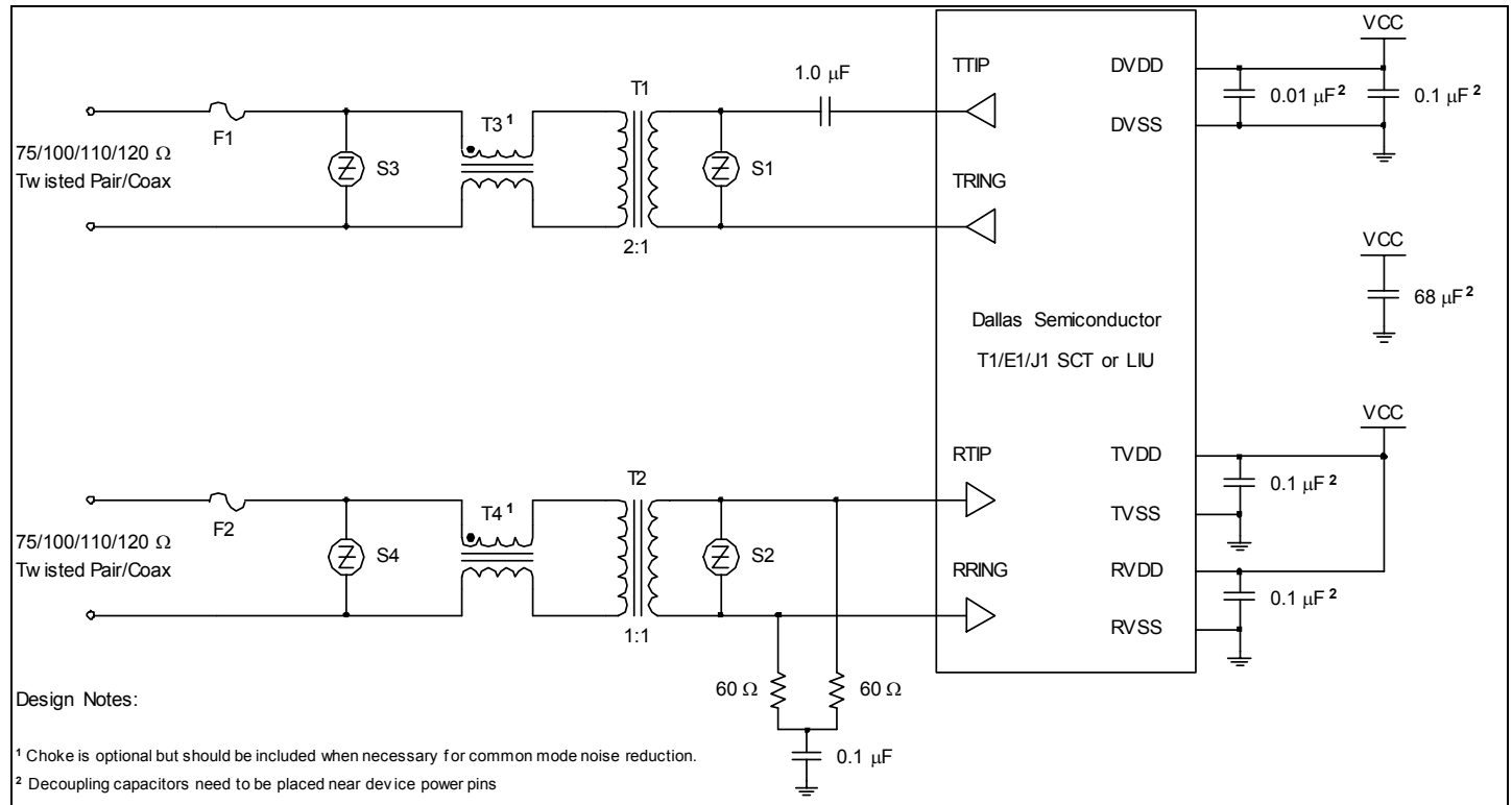
Figure 24-3. Software-Selected Termination, Metallic Protection
