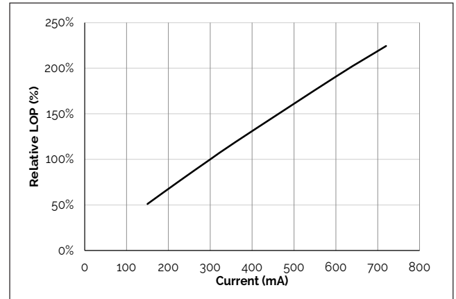
Figure 6: V10C Typical Relative Flux vs. Current
