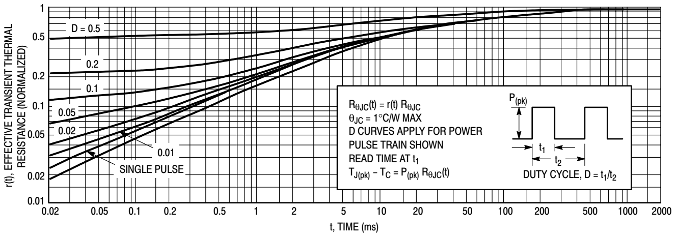
Figure 16. Thermal Response
